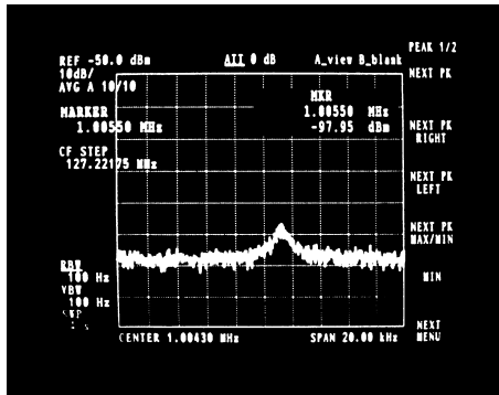
Figure: 5 ( f_{\beta_y} + f_{sh} ) of #1 bunch in 4th bunch train.
