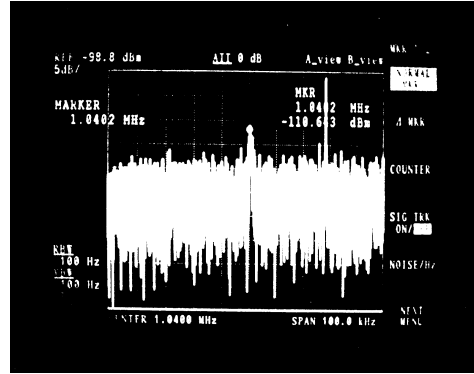
Figure: 4 Betatron sideband of the picked-out bunch. Middle peak corresponds to f_{\beta_y} + f_{\text{sh}} . Right-side peak corresponds to 2f_{\text{sh}} .
