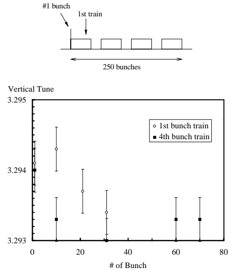
Figure: 7 Tunes of several bunches in the 1st and 4th bunch train. Error bars represent FWHM of spectral peaks.
