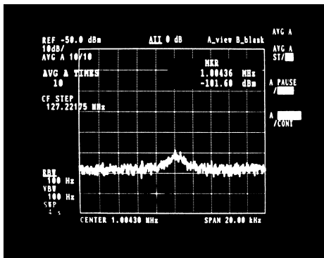
Figure: 6 ( f_{\beta_y} + f_{sh} ) of #70 bunch in 4th bunch train.
