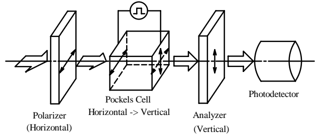
Figure: 1 Schematic diagram of high speed light shutter.
