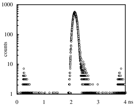
Figure: 3 Time structure of light passed through shutter.
