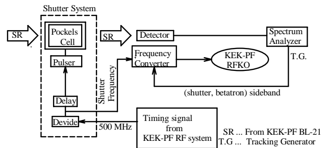
Figure: 2 Block diagram of bunch-by-bunch betatron oscillation detection system.
